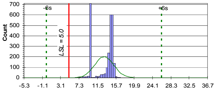
Old -55C Input Reverse Breakdown Voltage \times 10^0 Volts
