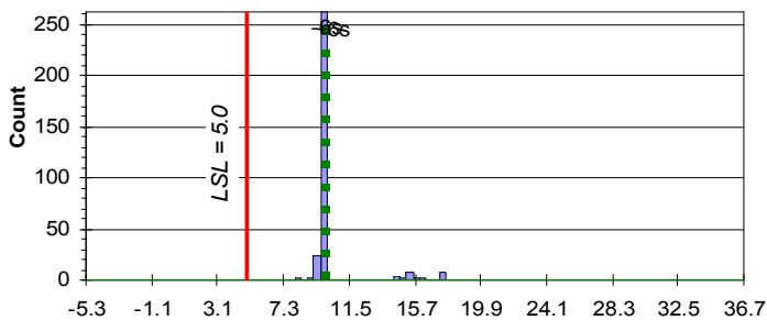
New +25C Input Reverse Breakdown Voltage \times 10^0 Volts
