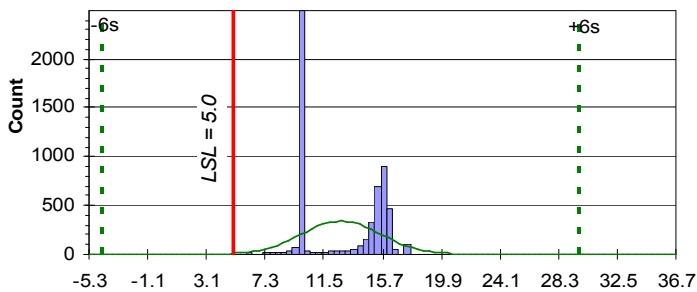
Old +25C Input Reverse Breakdown Voltage \times 10^0 Volts
